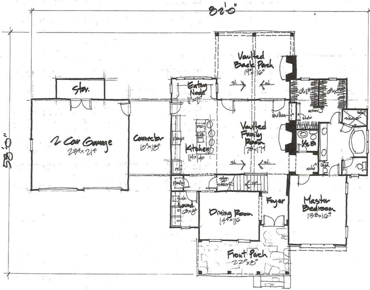
1st Floor Plan revised 07/20/10 9'6" dia. ± 1675 hooked up feet 50.14' x 16.0'
